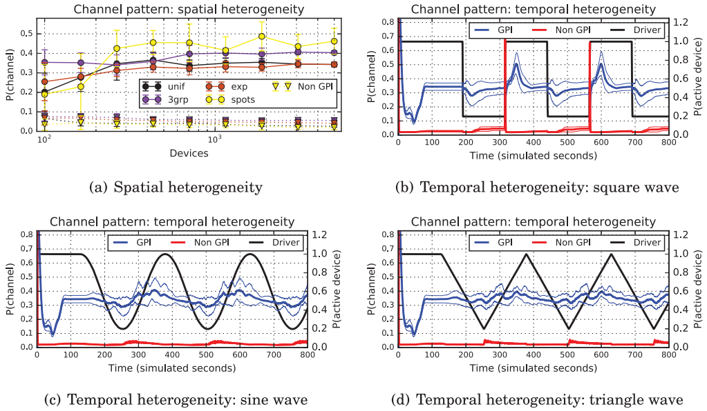
Fig. 12. Additional details of experimental data on wireless sensor network scenario confirming our predictions for GPI-calculus. Panel (a) compares GPI performance of Figure 8(c) with the non-GPI version (triangles). Panels (b)–(d) compare GPI performance of Figure 8(d) (blue) with the non-GPI version (red) for each of the three density driver waves (black). All graphs show mean and \pm 1 standard deviation for both GPI and non-GPI versions. As in the other tests in Figure 8, the non-GPI is disrupted by the fragility of floating point equality operations in every experiment. Results are the average of 10 simulation runs.
